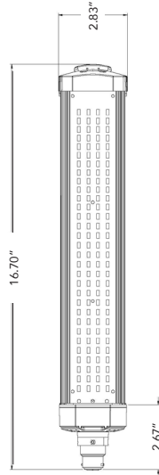
LED-8101 - 35W
